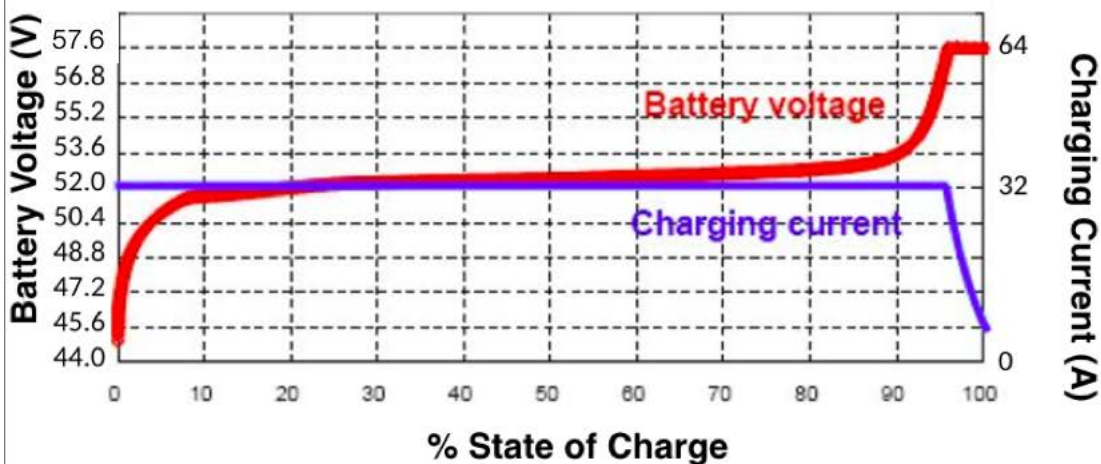
Voltage/Current Curve for charging LiFe12033P
